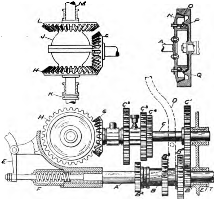
FIG. 349.—Details of the Panhard-Levassor Change Speed Gear. A is a square section of the main driving shaft connected to the motor by the cone clutch shown in the right hand upper diagram of the figure. B is a sleeve caused to slide on A by means of lever, D, which carries four spur pinions, B 1 , B 2 , B 3 , B 4 , which are of such diameter as to match respectively with pinions, C 1 , C 2 , C 3 , C 4 , keyed on the counter shaft, C. The motion being imparted from the main shaft, A, through sleeve, B, through any one pair of pinions to the shaft, C, causes the rotation of the bevel pinion, G, which, as shown in the left-hand upper diagram of the figure, may mesh with either bevel gear, H or L, which are secured to a sleeve sliding on a feather on shaft, M. At K is shown the spool to which is connected the fork of the shifting lever, the object being to alter the direction of the motion according as H or L is in gear. J is a differential gear drum. The main clutch is thrown on or off by means of the lever, E, and is held in position by the spring, F. The construction of the clutch shown is as follows: On the end of the shaft, A, are mounted the double male cones, N and P. On the end of the crank shaft of the engine are the double female cones, O and Q. When under the force of the spring, F, the two cones adhere by friction contact, thus transmitting the motion of the crank shaft to the main shaft, A, by throwing out the clutch, the engine may continue moving without driving the carriage.
